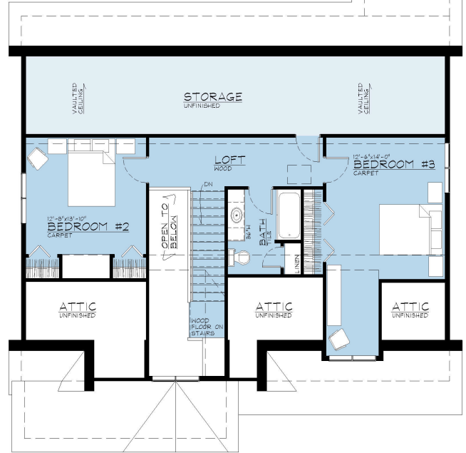
SECOND LEVEL PLAN
