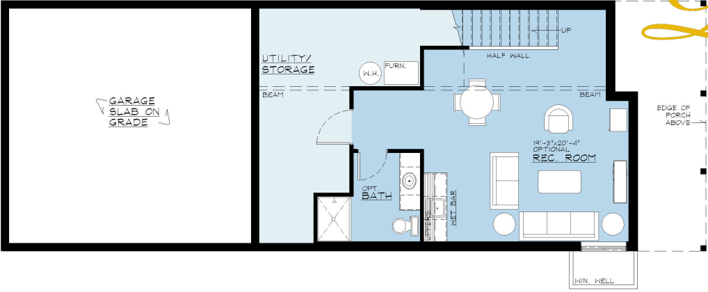
OPTIONAL FINISHED LOWER LEVEL PLAN
