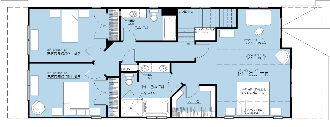
SECOND LEVEL PLAN
