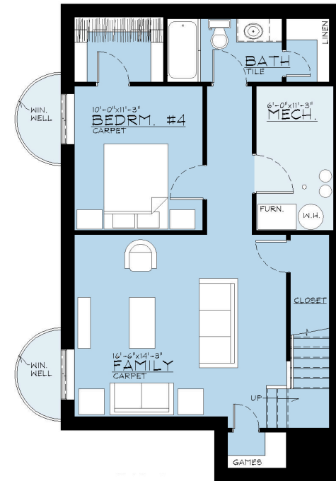
LOWER LEVEL PLAN
