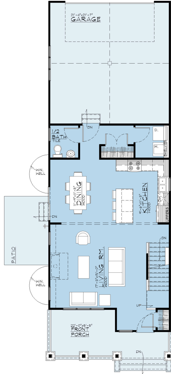
MAIN LEVEL PLAN
