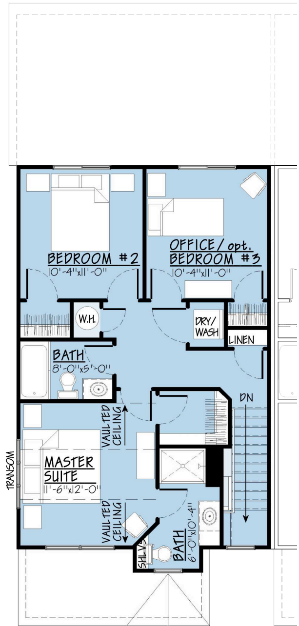
Second Level Plan
