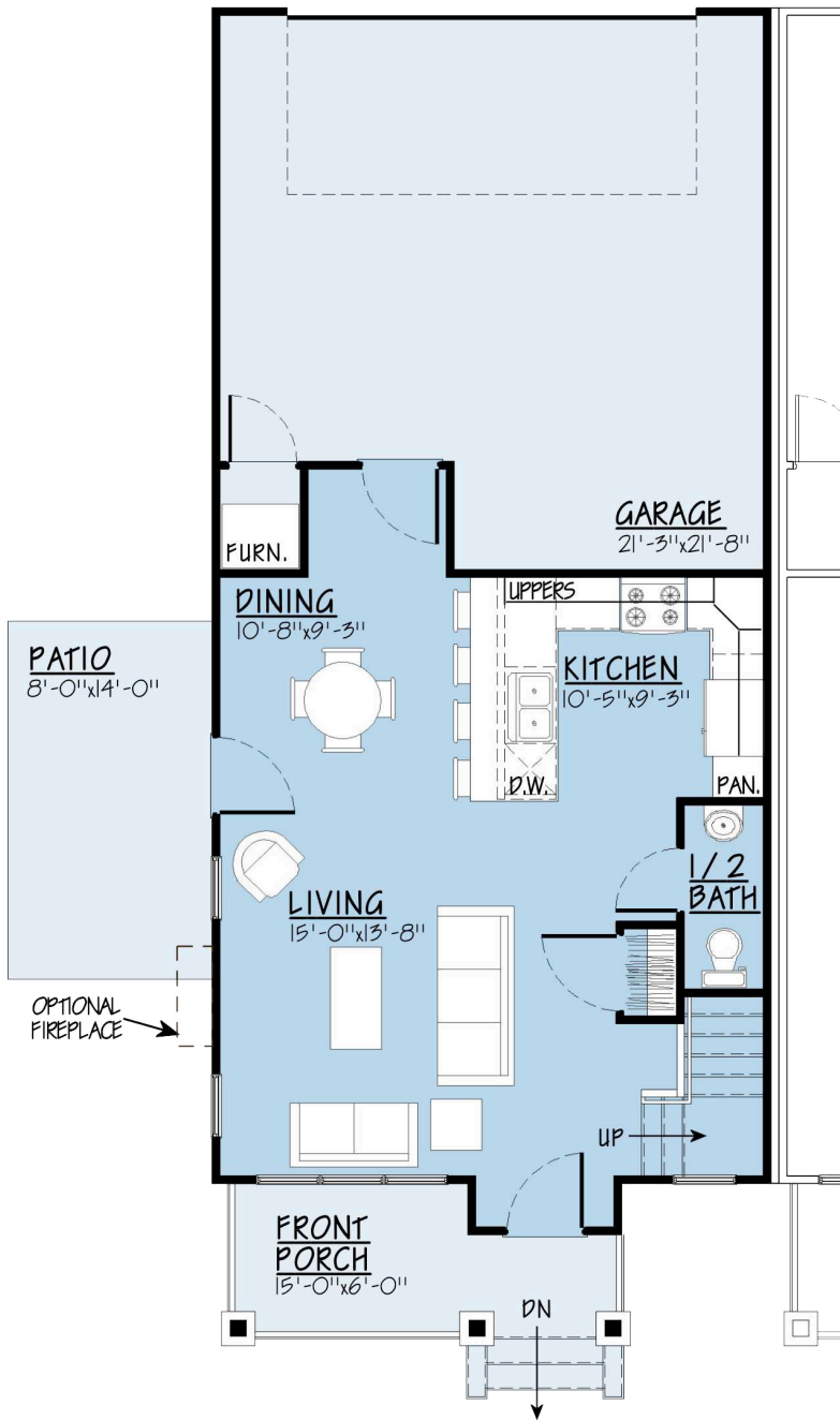
Main Level Plan
