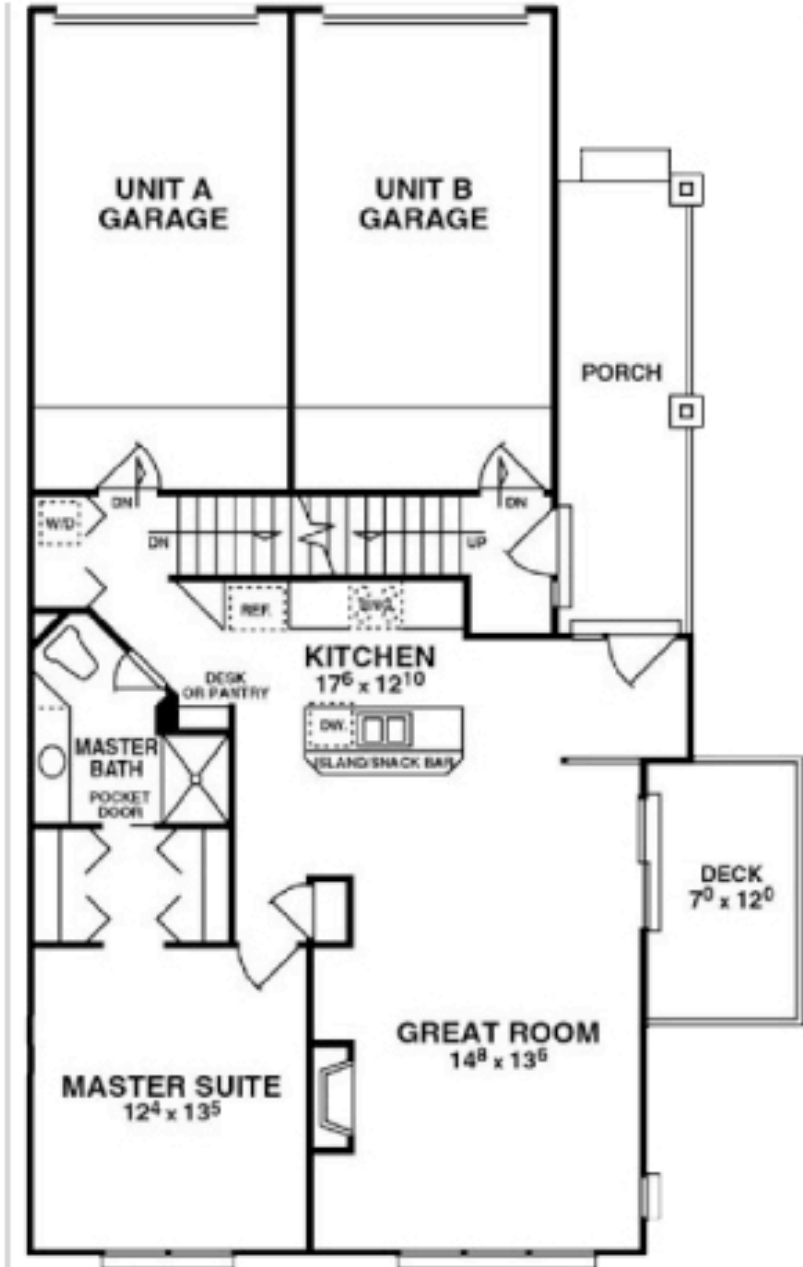
FIRST FLOOR PLAN UNIT A
