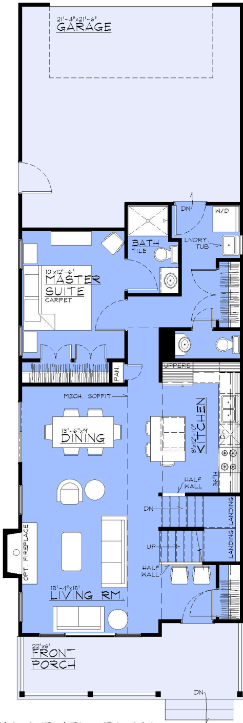
MAIN LEVEL PLAN
